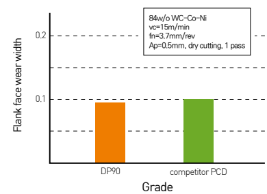
Continuous cutting test(workpiece:Al-25%Si)
